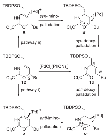
Scheme 9. The possible pathways for the conversion of ( S )- 13 into ( S,E )- 13 .
