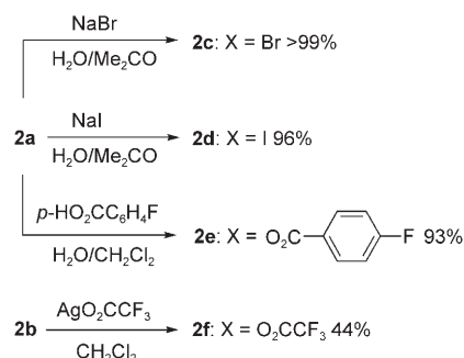
Scheme 3. Synthesis of additional derivatives of COP-X.
