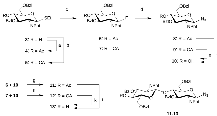
Scheme 2. a) \text{Ac}_2\text{O} /pyridine (quant.); b) chloroacetic anhydride/pyridine, \text{CH}_2\text{Cl}_2 (93 %); c) HF/pyridine, NBS, \text{CH}_2\text{Cl}_2 (93 % 6 ), (96 % 7 ); d) \text{TMS-N}_3 , \text{BF}_3 \cdot \text{OEt}_2 , \text{CH}_2\text{Cl}_2 (91 % 8 ), (92 % 9 ); e) MeOH, dioxane, NaOMe (67 %); f) \text{K}_2\text{CO}_3 , MeOH, \text{CH}_2\text{Cl}_2 (92 %); g) \text{BF}_3 \cdot \text{OEt}_2 , \text{CH}_2\text{Cl}_2 (83 %); h) \text{BF}_3 \cdot \text{OEt}_2 , \text{CH}_2\text{Cl}_2 (86 %); i) \text{K}_2\text{CO}_3 , MeOH, dioxane (79 %); k) \text{K}_2\text{CO}_3 , MeOH, \text{CH}_2\text{Cl}_2 (94 %).
