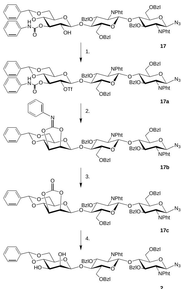
Scheme 5. 1) \text{TiF}_2\text{O} , pyridine, \text{CH}_2\text{Cl}_2 ; 2) DMF, pyridine, 65^\circ\text{C} ; 3) AcOH, dioxane, water; 4) NaOMe, MeOH, \text{CH}_2\text{Cl}_2 (overall yield 70 %).
