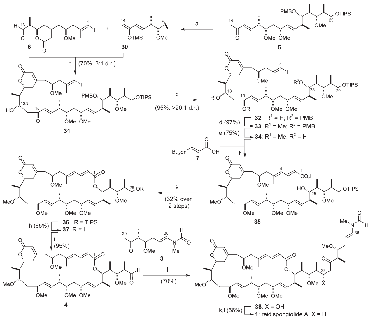
Scheme 5. Subunit assembly and completion of reidispongolide A. a) LDA, TMSCl, Et 3 N, THF, –78 °C; b) BF 3 ·Et 2 O, CaH 2 , CH 2 Cl 2 , –95 to –78 °C; c) Me 4 NBH(OAc) 3 , MeCN, AcOH, –30 °C; d) Me 3 O·BF 4 , proton sponge, CH 2 Cl 2 , 0 °C; e) DDQ, pH 7 buffer, CH 2 Cl 2 ; f) [Pd 2 (dba) 3 ], iPr 2 NEt, NMP; g) 1. 2,4,6-Cl 3 (C 6 H 2 )COCl, Et 3 N, PhMe; 2. DMAP; h) HF·py, py, THF; i) DMP, CH 2 Cl 2 ; j) 1. cHex 2 BCl, Et 3 N, Et 2 O, 0 °C; 2. 4, –78 to 0 °C, 1 h; k) Et 3 NSO 2 NCO 2 Me, THF; l) [(Ph 3 PCuH) 6 ], PhMe, H 2 O. LDA = lithium diisopropylamide, DDQ = 2,3-dichloro-5,6-dicyano-1,4-benzoquinone, dba = dibenzylideneacetone, NMP = 1-methyl-2-pyrrolidinone.
