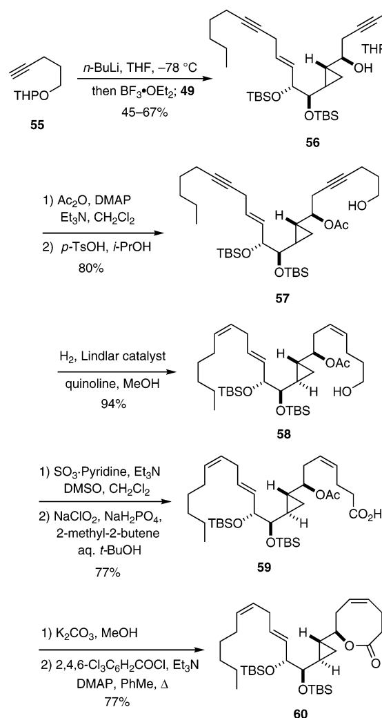
SCHEME 12
