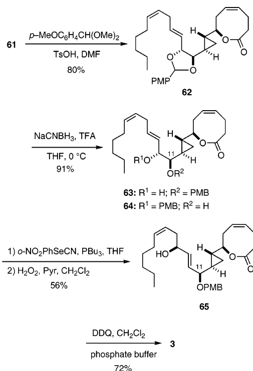
SCHEME 13
