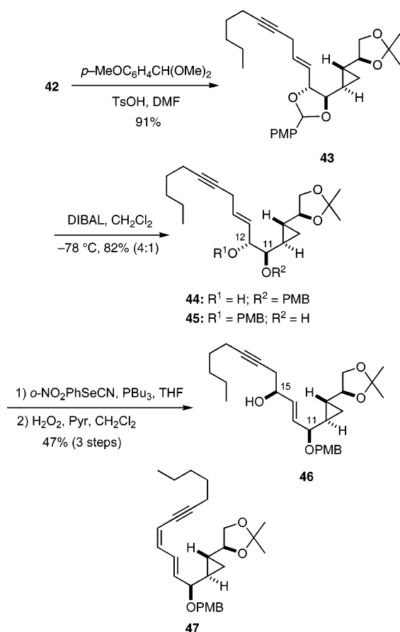
SCHEME 10
