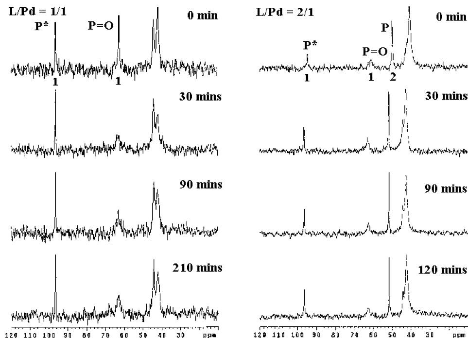
Figure 5. ^{31}\text{P} NMR spectra monitored from the reaction of 4a with \text{Pd}(\text{OAc})_2 in \text{THF-}d_8 at 40^\circ\text{C} . P: 4a , \text{P}=\text{O} : 4b , \text{P}^* : unknown. Left: 4a / \text{Pd}(\text{OAc})_2 = 1:1 ; Right: 4a / \text{Pd}(\text{OAc})_2 = 2:1 .
