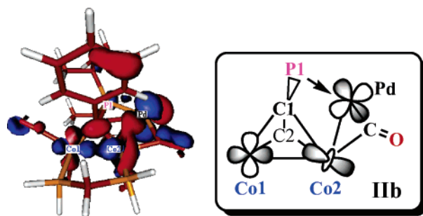
Figure 8. Localized Kohn–Sham orbital (B3LYP/6311LAN) of IIb (contour intervals: 0.025 in e·au –3 ) and schematic orbital interactions.
