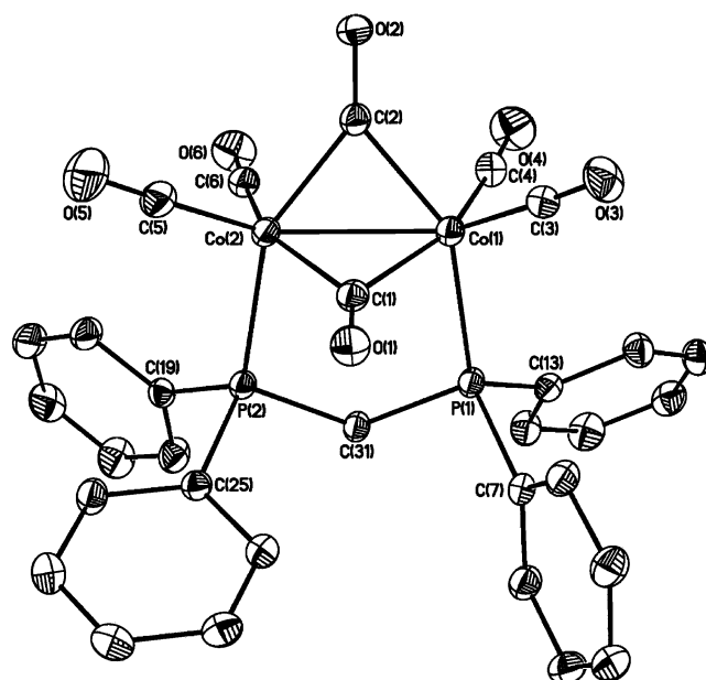
Figure 2. Molecular structure of (μ-PPh 2 CH 2 PPh 2 )Co 2 (CO) 6 , 3 . Hydrogen atoms are omitted for clarity. Selected bond lengths (Å) and angles (deg): Co(1)–Co(2) 2.4568(5), Co(1)–P(1) 2.2658(7), Co(2)–P(2) 2.2388(7), Co(1)–C(1) 1.953(3), Co(1)–C(2) 1.946(3), Co(2)–C(1) 1.933(3), Co(2)–C(2) 1.921(3), P(1)–Co(1)–Co(2) 97.27(2), P(2)–Co(2)–Co(1) 99.96(2), P(2)–C(31)–P(1) 115.92(13).
