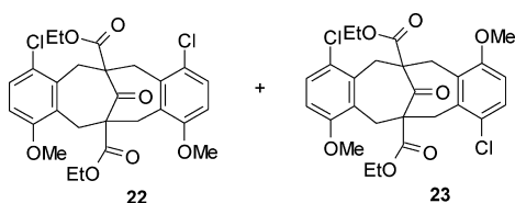
Figure 2. Dimerization impurities.
