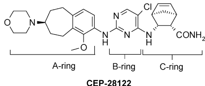
Figure 1. ALK inhibitor CEP-28122.
