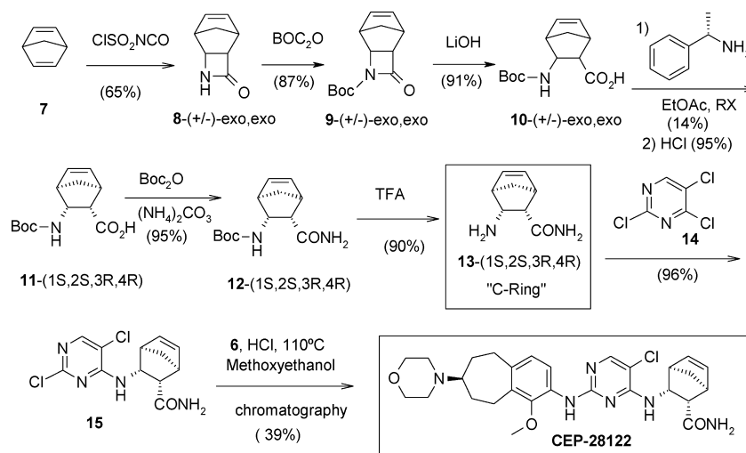
Scheme 2. Medicinal chemistry route to C-ring and CEP-28122
