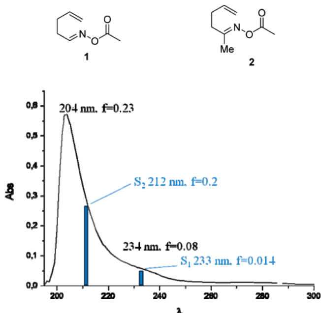
FIGURE 1. Calculated transitions (blue) for model 1 and experimental UV spectrum (black) for compound 2 .
