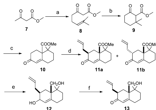
Scheme 2 Reagents and conditions: (a) NaH, n-BuLi, 4-bromo-2-methyl-2-butene, THF, 0^\circ\text{C} , 79%; (b) \text{SnCl}_4 , \text{CH}_2\text{Cl}_2 , r.t., 81%; (c) \text{KOCH}_3 , MVK, 0^\circ\text{C} ; \text{K}_2\text{CO}_3 , \text{CH}_3\text{OH} , reflux, 80%; (d) LDA, allylic bromide, -78^\circ\text{C} \rightarrow \text{r.t.} , 63% ( 11a ), 9% ( 11b ); (e) \text{LiAlH}_4 , THF, r.t., 76%; (f) DDQ, benzene, r.t., 70%.
