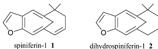
Fig. 1 Structures of spiniferin-1 and dihydrospininiferin-1.
