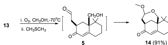
Scheme 3 The confirmation of relative configuration of 11a .
