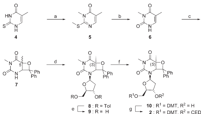
Scheme 1. Synthesis of the oxetane electron acceptor 2 . a) MeI, DMF, RT, 18 h, 65%; b) 3N HCl, 80 °C, 8 h, 93%; c) hν , benzophenone, MeCN, 3 h, 44%; d) \alpha -1'-chloro-3',5'-di- O -toluoyl-deoxyribofuranoside, NaH, MeCN, RT, 4 h, 53% \alpha/\beta 1:1; e) K_2CO_3 , MeOH, RT, 3 h, 84%; f) DMTCl, pyridine, RT, 4 h, 84%; g) \beta -cyanoethyltetraisopropylphosphordiamidite, diisopropylethylamine, THF, RT, 2 h, 67%.
