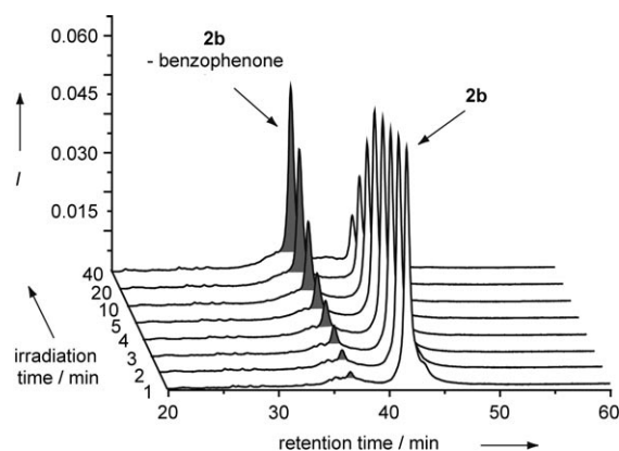
Figure 5. HPLC traces obtained during the irradiation experiment with hairpin 2b . Assay solution: Hairpin concentration = 20 μM in buffer (150 mM NaCl, 10 mM Tris-HCl, 9.8 mM Na 2 S 2 O 4 , pH 7.4). Irradiation with 1000 W xenon lamp, cut-off filter λ = 340 nm, T = 20°C. HPLC conditions: Nucleosil column (120 Å, 3 μm); eluting buffers (buffer A: 0.1 M NH 4 Et 3 OAc in H 2 O; buffer B: 0.1 M NH 4 Et 3 OAc in MeCN); Gradient: 0–10% B in 10 min and then up to 45% B in 45 min at a flow of 0.5 mL min −1 . I = relative absorbance.
