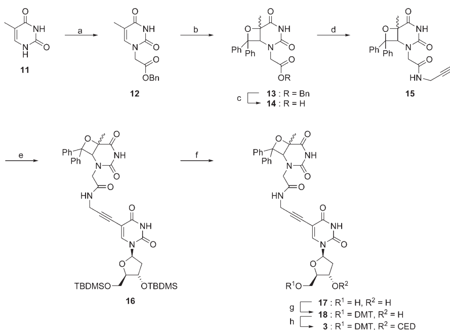
Scheme 2. Synthesis of the oxetane acceptor 3 . a) benzyl bromoacetate, K 2 CO 3 , DMF, RT, 0°C → RT, 20 h, 68%; b) hν , benzophenone, MeCN, RT, 5 h, 57%; c) H 2 , Pd/C, EtOAc, RT, 3 h, 98%; d) propargylamine, HOBt, TBTU, NEt 3 , DMF, RT, 86%; e) 5-iodo-3',5'-di- O -TBDMS-deoxyuridine, CuI, [PdCl 2 (PPh 3 ) 2 ], DIEA, DMF, RT, 12 h, 66%; f) HF-pyridine, pyridine, THF, RT, 12 h, then MeOTMS; g) DMTCl, 4-DMAP, pyridine, mol sieves 4 Å, RT, 54 h, 41% over two steps; h) β-cyanoethyltetraisopropylphosphordiamidite, diisopropylammonium tetrazolate, dichloromethane, RT, 12 h, 58%.
