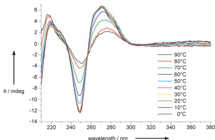
Figure 4. Temperature dependent CD spectra of the hairpin 3a . Conditions: Hairpin concentration = 3 μM in buffer (150 mM NaCl, 10 mM Tris-HCl, pH 7.4).
