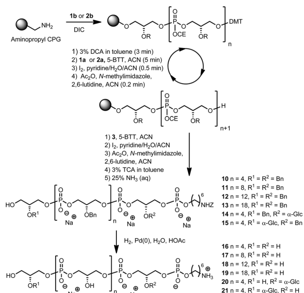
Scheme 2 Automated solid phase TA synthesis.
