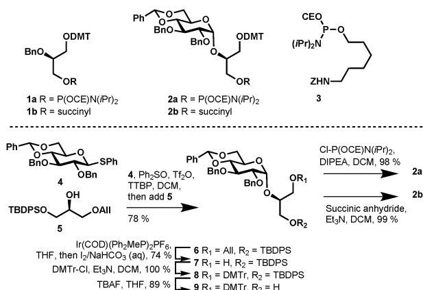
Scheme 1 Building blocks for the automated solid phase TA synthesis.
