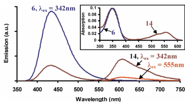
Fig. 4 Emission spectra of 6 ( \lambda_{\text{ex}} = 342 \text{ nm} ) and 14 ( \lambda_{\text{ex}} = 342 and 555 \text{ nm} ) in \text{CHCl}_3 at rt. Inset: Absorption spectra of 6 and 14 in \text{CHCl}_3 at rt.
