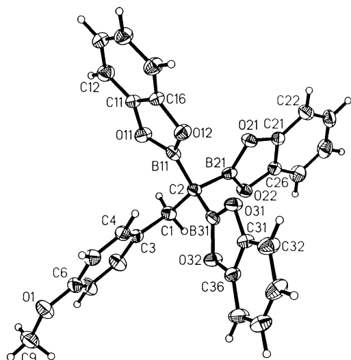
Fig. 2. Molecular structure of one of the two independent molecules in the asymmetric unit of 2b . Ellipsoids shown at 50% probability for non-H atoms, with H atoms shown as circles of arbitrary radius.
