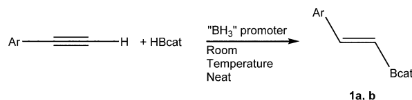
Equation (1). ' \text{BH}_3 ' promoted hydroboration of ethynylarenes.
