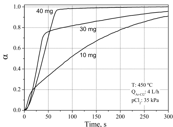
Figure 11. Effect of the mass sample on the kinetics of \text{La}_2\text{O}_3 chlorination at 450 °C.
