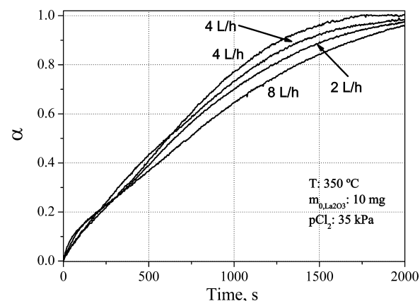
Figure 9. Effect of \text{Ar-Cl}_2 flow rate on the kinetics of \text{La}_2\text{O}_3 chlorination at 350 °C. Two curves of 4 L/h are presented to show the reproducibility of the system.
