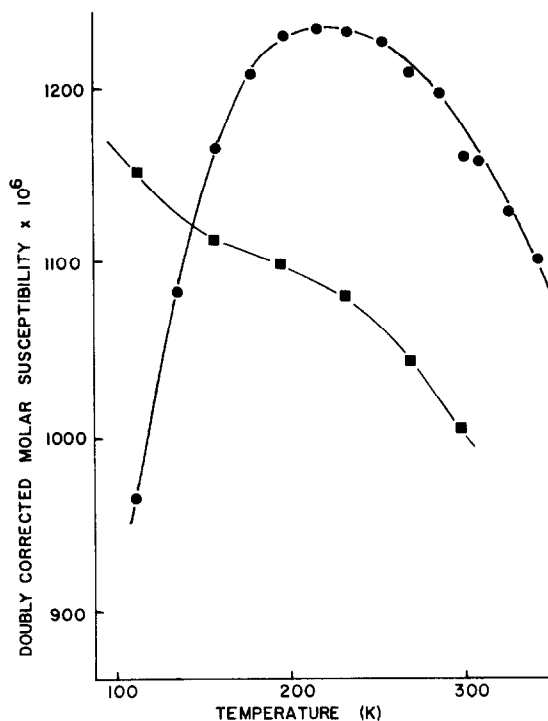
Fig. 3. Plot of the doubly corrected molar susceptibility of anhydrous \text{Cu}(\text{npaa})_2 versus temperature. The circles represent preparation A and the squares preparation B.
