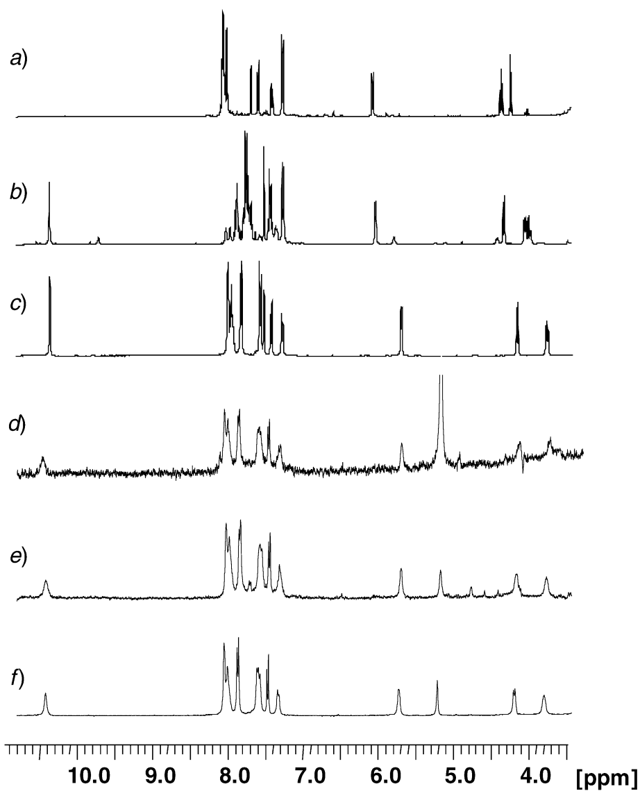
Fig. 3. 1 H-NMR Spectra ((D 6 )DMSO) of a) 14 , b) 15 , and c) 16 , and 1 H-NMR Spectra ((D 6 )DMSO) resulting from d) 14 , e) 15 , and f) 16 after incubation of separate samples in phosphate buffer and lyophilization showing the presence of 16 only (cf. c)
