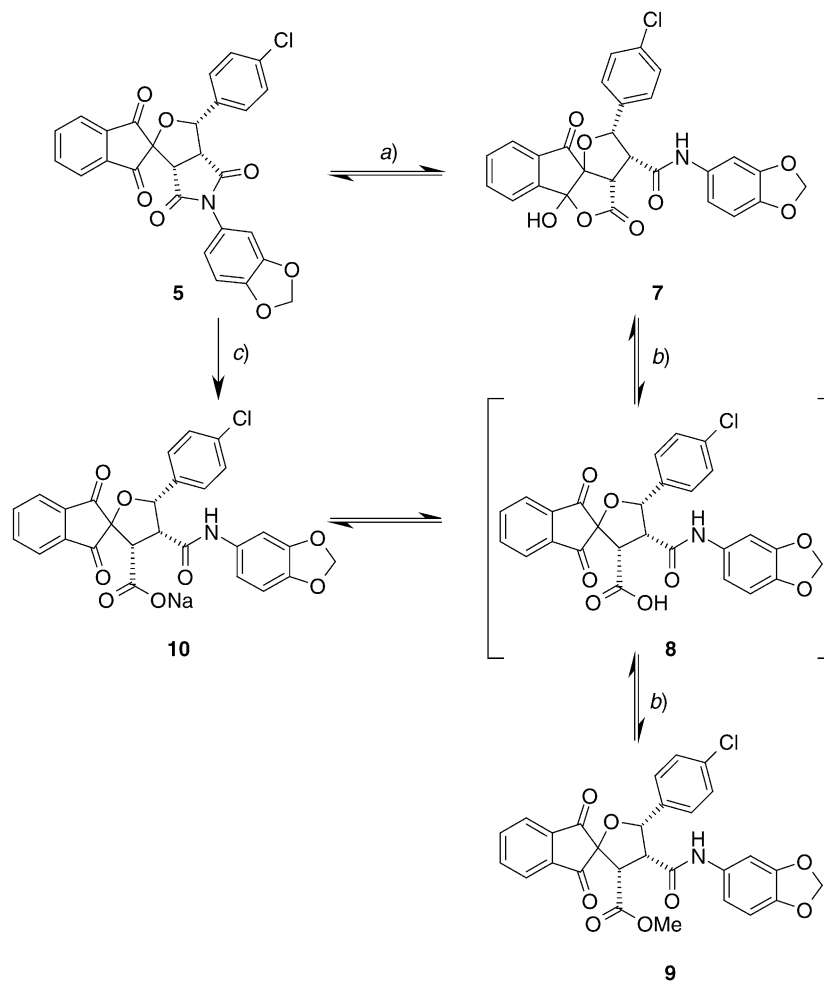
Scheme 2. Maleimide Hydrolysis
