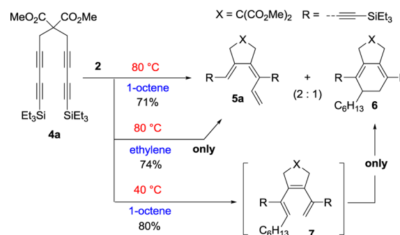
Scheme 1. Influence of Temperature and Alkene Structure on Metathesis versus 1,4-Hydrovinyllative Cyclization
