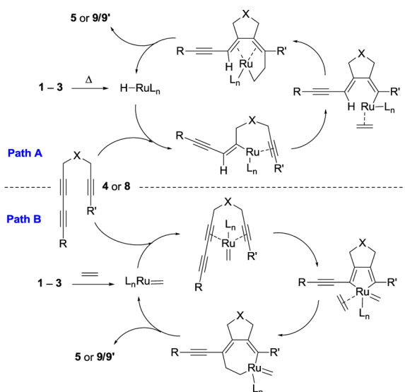
Scheme 2. Two Plausible Mechanisms
