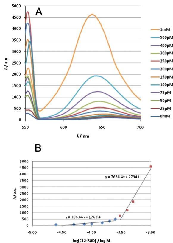
Fig. 3 A) Nile Red fluorescence emission spectra in the presence of increasing concentrations of C12-RGD. B) Fluorescence emission intensities of Nile Red at 635 nm plotted against log[C12-RGD] in order to determine the Critical Aggregation Concentration (CAC). Excitation wavelength: 550 nm.
