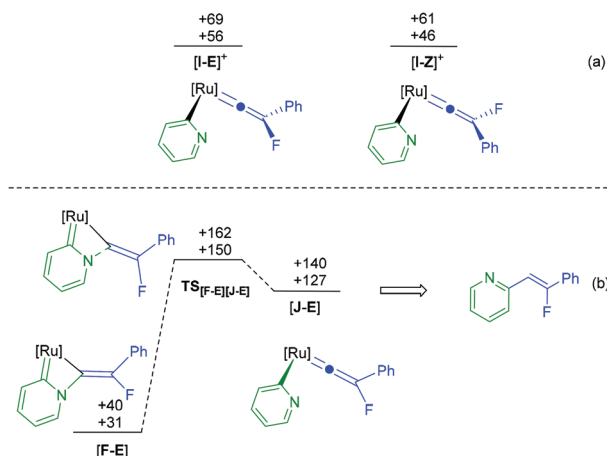
Fig. 6 Calculations at the (RI)-PBE0-D3/def2-TZVPP//[(RI)-BP86/SV(P)] level with COSMO solvation in pyridine. [Ru] = [Ru(\eta^5-C_5H_5)(PPh_3)] . E_{SCF+ZPE} (top) and Gibbs energies at 298.15 K (bottom), relative to [3a]^+ , pyridine and PPh_3 .
