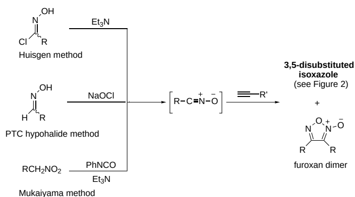
Figure 5. Methods of nitrile oxide generation.
