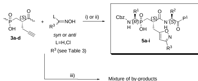
Scheme 4. Methods for the preparation of the isoxazole-containing phosphinic pseudopeptides of type 5 . i) Method A (one-flask procedure): L = H, oxime (6 equiv) in CHCl 3 , pyridine(cat.), NCS (6 equiv), 45 °C, 3–4 h, then 3a–d , Et 3 N (7 equiv, portionwise), 45 °C, 48–60 h. ii) Method B (two-step procedure): L = Cl, oxime (6 equiv) in DMF, NCS (6 equiv), 45 °C, 40 min, isolation of the hydroximinoyl chloride, then 3a , Et 3 N (7 equiv, portionwise), RT, 48 h. iii) NaOCl aq , CH 2 Cl 2 , Et 3 N (cat.), RT, 12 h.
