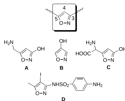
Figure 2. General structure of 3,5-disubstituted isoxazole core (top). Examples of naturally occurring and synthetic isoxazoles of pharmaceutical interest. A: Muscimol; [20] B: 4-hydroxyisoxazole; [20] C: ibotenic acid; [19d] D: selective endothelin receptor A (ET A ) antagonist. [19f]
