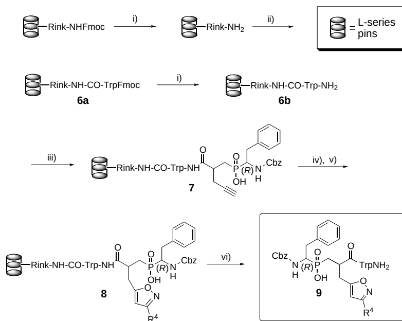
Scheme 5. Solid-phase synthesis of the isoxazole-containing phosphinic tripeptide array of type 9 : i) 20 % pip/DMF; ii) FmocTrpOH, DIC, HOBT, \text{CH}_2\text{Cl}_2 /DMF; iii) 2a or 2a' , EDC·HCl, HOBT, DIPEA, \text{CH}_2\text{Cl}_2 , RT, 2 h; iv) \text{R}^4\text{CH}=\text{NOH} (oxime), NCS, Py (cat.), \text{CHCl}_3 , 45 °C; v) \text{Et}_3\text{N} , 45 °C; vi) TFA/ \text{H}_2\text{O} /TIS (95:2.5:2.5).
