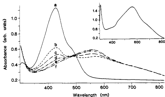
Figure 4. Overall UV-vis absorbance changes in the formation of \text{VPy}_4\text{H}_2 from \text{VPy}_4(\text{CF}_3\text{SO}_3)_2 in pyridine solvent: (a) spectrum of \text{V}(\text{Py})_4(\text{CF}_3\text{SO}_3)_2 at room temperature; (b) spectrum of the sample in (a) with \text{LiEt}_3\text{BH} ( \text{H}^-/\text{V}(\text{II}) ratio = 2.2; overnight reaction) at -20^\circ\text{C} ; (c-f) spectra recorded within 6 min while the solution from (b) warms to room temperature. The inset shows the optimum spectrum for \text{VPy}_4(\text{H})_2 .
