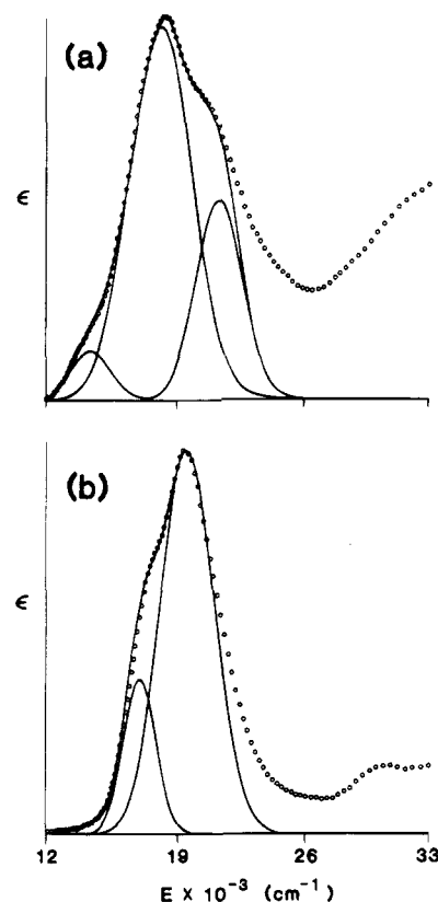
Figure 8. Gaussian resolutions of the room-temperature visible absorption spectra of VPy 4 (N 3 ) 2 (top frame) and VPy 4 (Cl) 2 (bottom frame). The symbols (○) represent the experimental absorption spectra.
