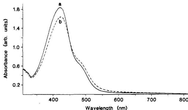
Figure 7. (a) Absorption spectrum of \text{VPy}_4(\text{CF}_3\text{SO}_3)_2 in pyridine. (b) Spectrum of the sample in (a) in the presence of 100 mol of \text{H}_2\text{O} /mol of \text{V(II)} (immediate response).
