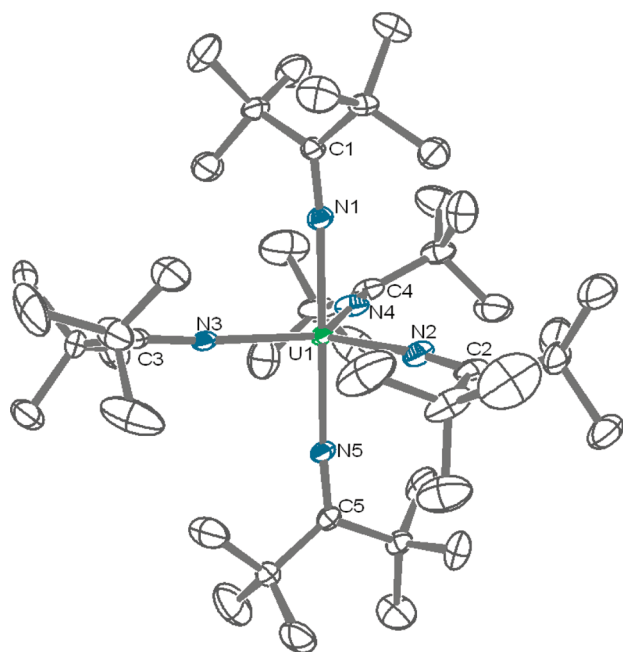
Figure 2. Solid-state molecular structure of \text{U}(\text{N}=\text{C}^t\text{Bu}_2)_5 (3) with 50% probability ellipsoids. Selected bond lengths (Å) and angles (deg): U1–N1 = 2.180(5), U1–N2 = 2.193(5), U1–N3 = 2.208(4), U1–N4 = 2.173(5), U1–N5 = 2.181(5), U1–N1–C1 = 172.6(4), U1–N2–C2 = 172.7(5), U1–N3–C3 = 175.2(4), U1–N4–C4 = 179.5(5), U1–N5–C5 = 175.3(4).
