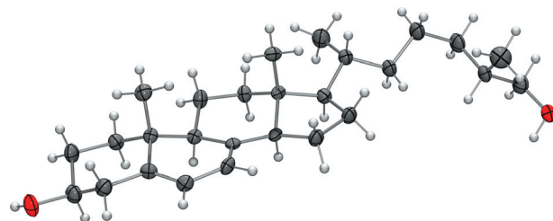
Fig. 3 Molecular structure of (25 S )-cholesta-5,7-diene-3 \beta ,26-diol ( 19 ) in the crystal (ORTEF plot at the 50% probability level).
