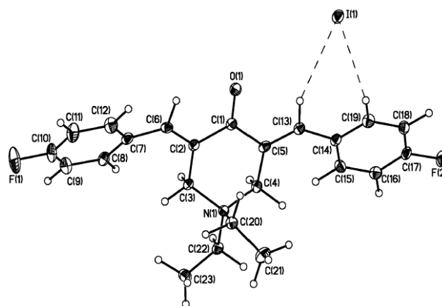
Figure 1. The general view of 4d in representation of atoms by thermal ellipsoid plots ( p=50\% ). The selected bond lengths (Å): O(1)-C(1) 1.224(3), N(1)-C(3) 1.505(3), N(1)-C(4) 1.508(3), N(1)-C(20) 1.514(3), N(1)-C(22) 1.524(3), C(1)-C(2) 1.485(4), C(1)-C(5) 1.486(4), C(2)-C(6) 1.340(4), C(5)-C(13) 1.349(4); bond angles (°): C(3)-N(1)-C(4) 108.7(2), C(2)-C(1)-C(5) 117.8(2), C(1)-C(2)-C(6) 116.7(2), C(1)-C(5)-C(13), 116.9(2).
