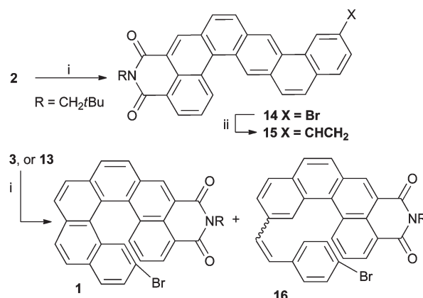
Scheme 2 Reagents and conditions: i, h\nu , \text{I}_2 , toluene, r.t.; ii, tributyl(vinyl)tin, \text{Pd}_2(\text{dba})_3 , \text{P}(\text{tBu})_3 , toluene, 80 °C (86%).
