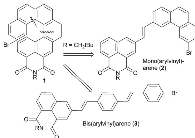
Fig. 1 Retrosynthetic approach to 1,8-naphthalimide with [6]helicene skeleton.
