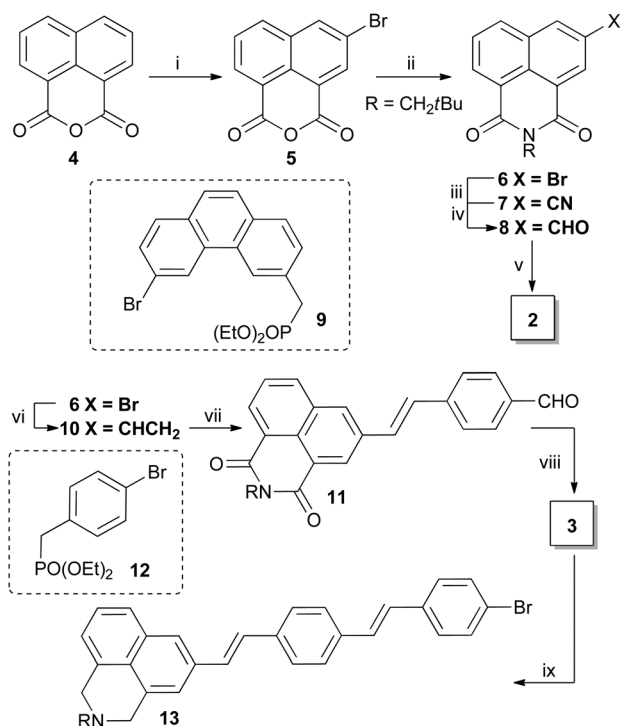
Scheme 1 Synthesis of mono(arylvinyl)arene 2 and bis(arylvinyl)arene 3 . Reagents and conditions: i, \text{Br}_2 , \text{Ag}_2\text{SO}_4 , \text{H}_2\text{SO}_4 , 65 °C (93%); ii, neopentylamine, dioxane, 100 °C (quant.); iii, \text{CuCN} , L-proline, DMF, 160 °C (82%); iv, RANEY® Ni, \text{HCO}_2\text{H} , reflux (29%); v, 9 , NaH, THF, 0 °C–r.t. (98%); vi, tributyl(vinyl)tin, \text{Pd}_2(\text{dba})_3 , \text{P}(\text{tBu})_3 , toluene, 80 °C (73%); vii, 4-bromobenzaldehyde, \text{Pd}(\text{OAc})_2 , \text{PPh}_3 , AcONa, DMF, 120 °C (96%); viii, 12 , NaH, THF, 0–30 °C (79%); ix, \text{LiAlH}_4 , \text{AlCl}_3 , THF, 0 °C–r.t. (76%).
