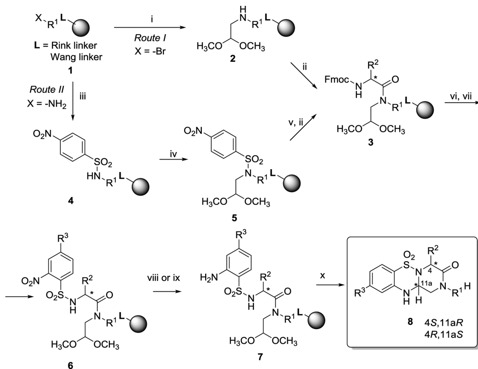
Scheme 2. Solid-Phase Stereoselective Synthesis of Tetrahydrobenzopyrazino-thiadiazinone Dioxides 8 a
