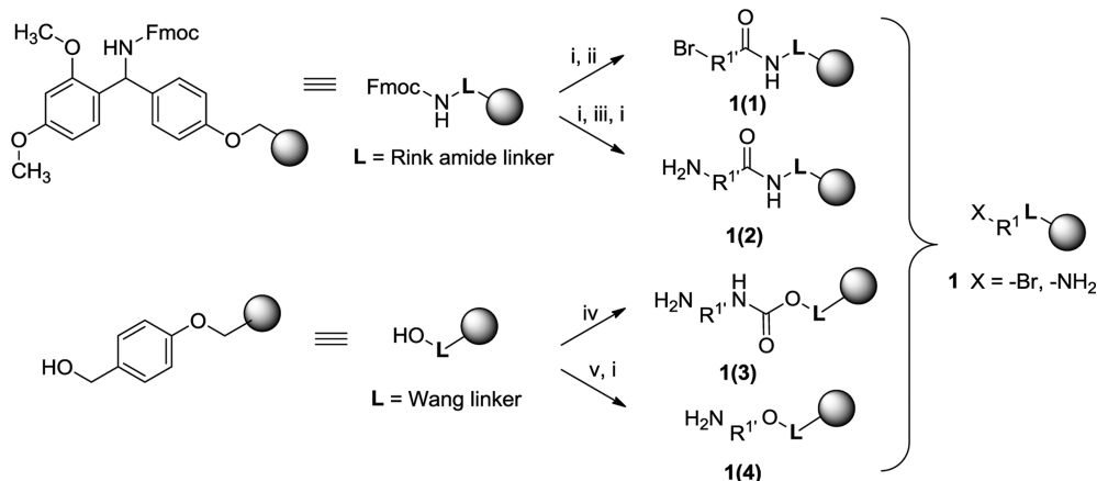
Scheme 1. Immobilization of the First Building Blocks on a Polymer Support a
