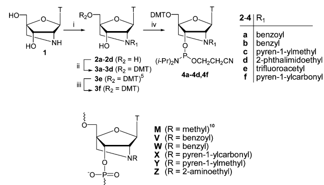
Fig. 1 Average structure from molecular dynamics simulation. Stereo view of a fully modified nonamer N -benzoyl 2'-amino-LNA [5'-(MeCTGA-TATGMeC)]-RNA hybrid viewed into the minor groove. For clarity, no hydrogens are shown. The colouring scheme is: nucleobases, yellow; sugar-phosphate backbone, red; benzoyl moieties, blue.
