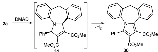
Scheme 4 Synthesis of pyrrolodibenzazepine 30 .
