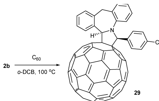
Scheme 3 Synthesis of fulleropyrrolidine 29 .
