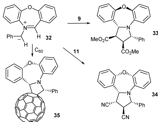
Scheme 5 Cycloaddition of ylide 32 .
