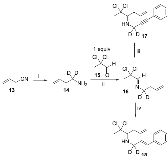
Scheme 4. Deuterium labelling strategy. Reagents and conditions: (i) \text{AlCl}_3 (1 equiv), \text{LiAlD}_4 (1 equiv), \text{Et}_2\text{O} , 0^\circ\text{C} , 1.5 h (19%); (ii) anhydrous \text{MgSO}_4 (3 equiv), \text{CH}_2\text{Cl}_2 , reflux, 2 h (37%); (iii) 7 (1 equiv), \text{BF}_3 \cdot \text{Et}_2\text{O} (1 equiv), \text{CH}_2\text{Cl}_2 , rt, 18 h (17%); (iv) 8 (1 equiv), \text{BF}_3 \cdot \text{Et}_2\text{O} (1 equiv), \text{CH}_2\text{Cl}_2/\text{HFIP} (9/1), rt, 18 h (7%).
