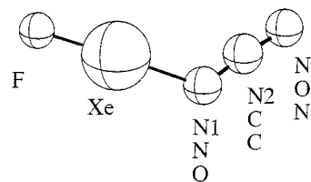
Figure 1. Structures of FXeN 3 , FXeNCO, and FXe(OCN).
