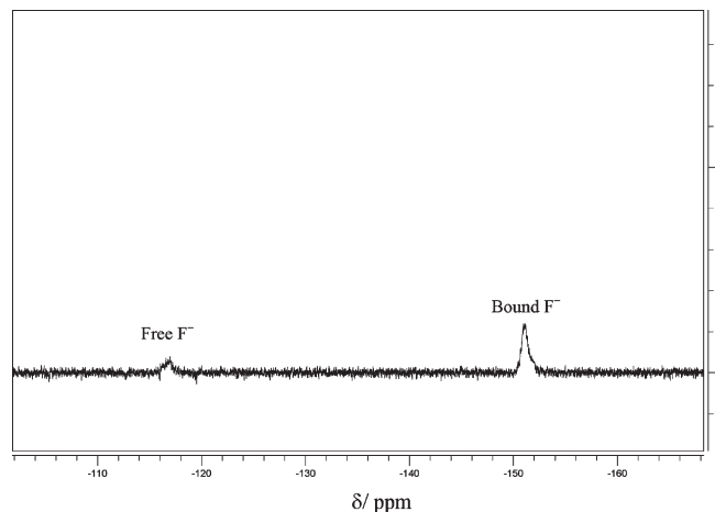
Figure 6. 19 F NMR spectrum of 1 in the presence of an excess of t Bu 4 NF in CD 3 CN.
