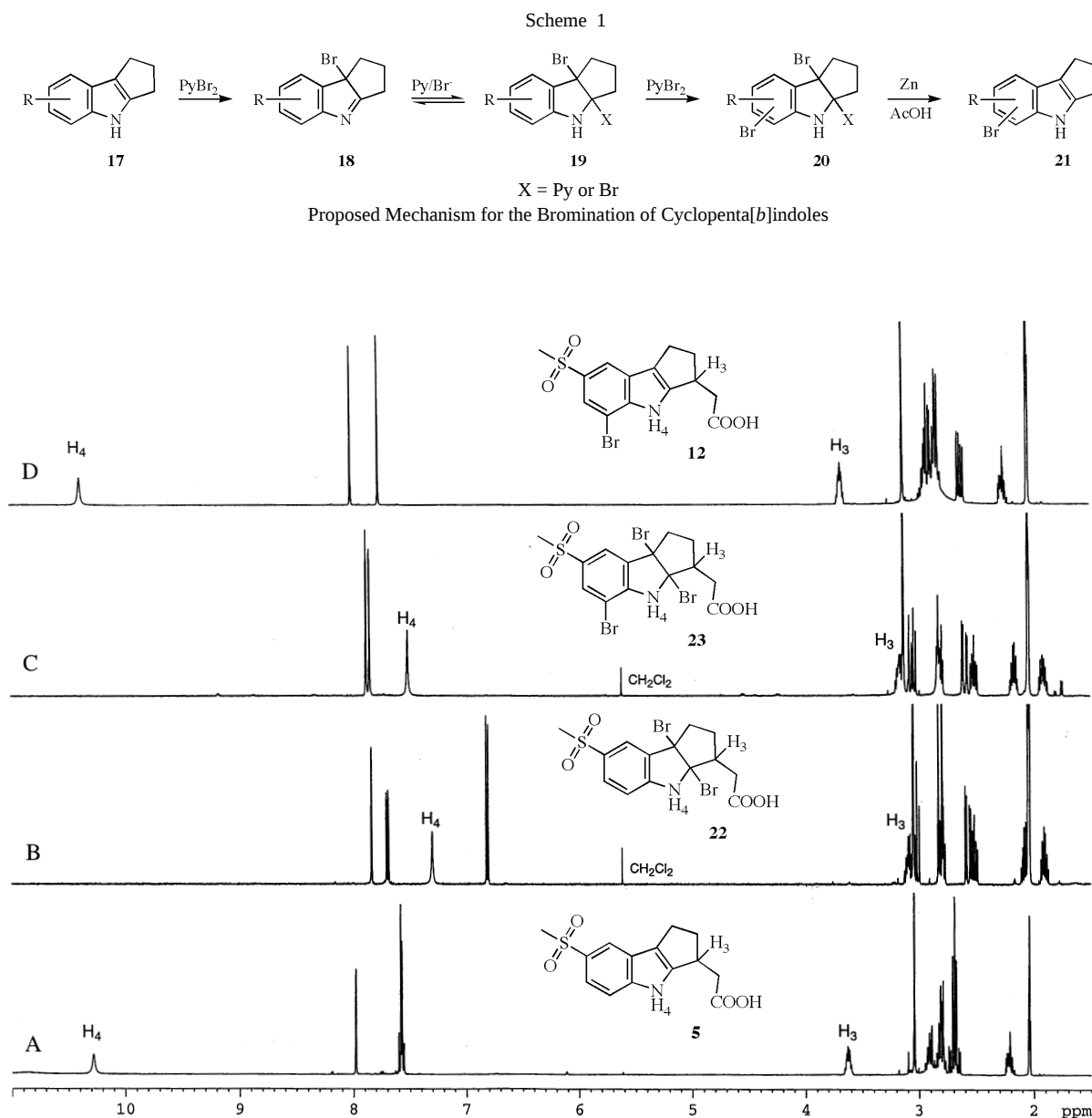
Figure 2. Crude ^1\text{H} nmr (500 MHz, acetone- d_6 ) of the bromination reaction of cyclopenta[b]indole 5 followed by the reduction of the intermediates 22 and 23 formed: (A) cyclopenta[b]indole 5 , (B) indoline 22 after the addition of 1 equiv of \text{PyBr}_2 at -20\text{ }^\circ\text{C} , (C) indoline 23 after the addition of excess \text{PyBr}_2 at 0\text{ }^\circ\text{C} , (D) bromocyclopenta[b]indole 12 after the addition of Zn and AcOH.
