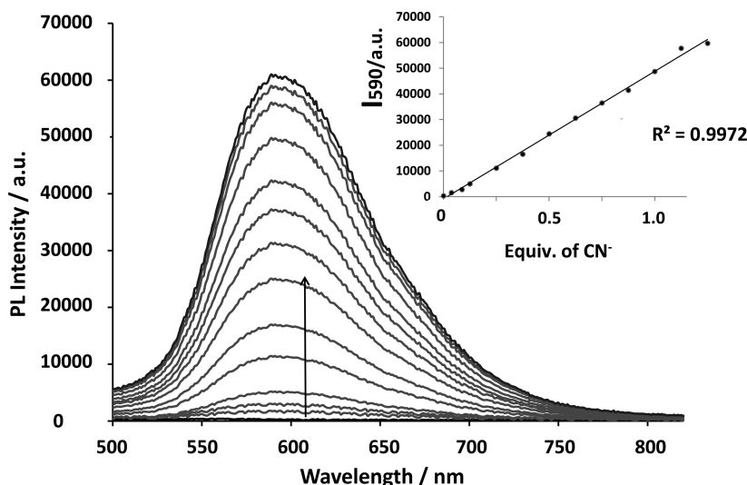
Figure 2. Changes in photoluminescence intensity of 1 ( 2.0 \times 10^{-5} M in \text{CH}_2\text{Cl}_2 ) upon the addition of cyanide ( (0\text{--}2.4) \times 10^{-5} M n\text{-Bu}_4\text{NCN} ). Inset shows luminescence titration of 1 ( 2.0 \times 10^{-5} M) with n\text{-Bu}_4\text{NCN} in \text{CH}_2\text{Cl}_2 at 293 K. [n\text{-Bu}_4\text{NCN}] = (0, 0.06, 0.1, 0.2, 0.3, 0.6, 0.8, 1.0, 1.2, 1.6, 2.0, 2.2, 2.4) \times 10^{-5} M; \lambda_{\text{ex}} = 413 nm.
