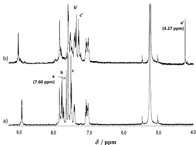
Figure 3. Partial ^1\text{H} NMR ( \text{CD}_2\text{Cl}_2 , 300 MHz) spectra of 1 (a) and that upon titration of 1 equiv of cyanide ions (as n\text{-Bu}_4\text{N}^+ salt) (b).
