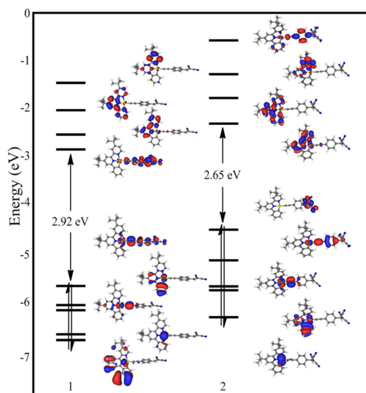
Figure 4. MO diagrams of 1 and 2 .
