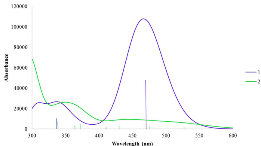
Figure 5. Computed absorption spectra of 1 and 2.
