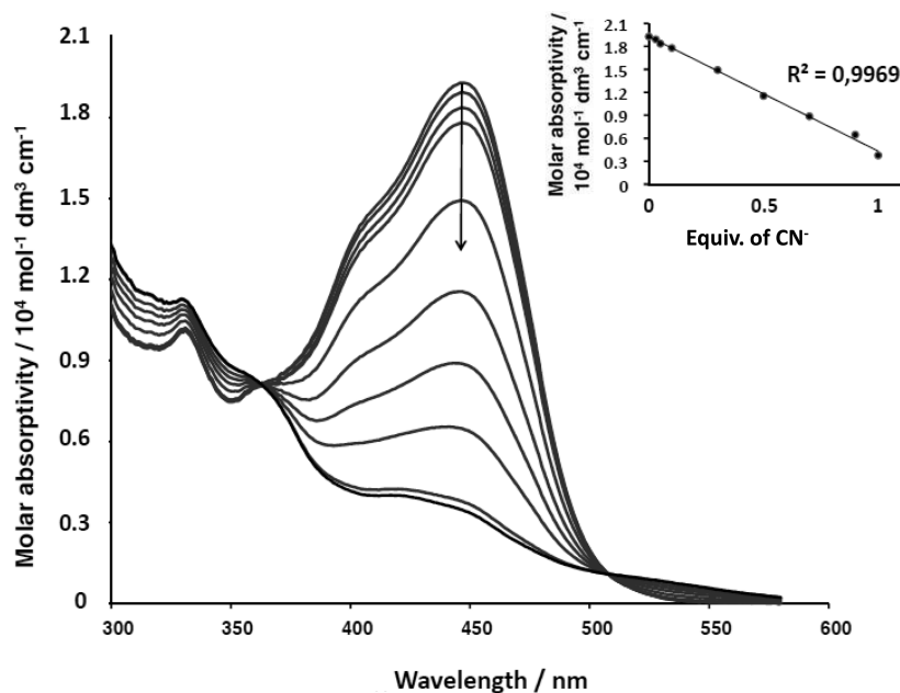
Figure 1. Changes in the UV–vis absorption spectrum of 1 ( 2.0 \times 10^{-5} M in \text{CH}_2\text{Cl}_2 ) upon the addition of cyanide ( (0\text{--}2.0) \times 10^{-5} M). Inset shows the absorption titration of 1 ( 2.0 \times 10^{-5} M) at 450 nm with addition of n\text{-Bu}_4\text{NCN} in \text{CH}_2\text{Cl}_2 at 293 K. [n\text{-Bu}_4\text{NCN}] = (0, 0.06, 0.1, 0.2, 0.6, 0.8, 1.0, 1.2, 1.6, 2.0) \times 10^{-5} M.
