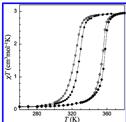
Figure 1. Temperature dependence of the product \chi T on cooling (empty symbols) and heating (full symbols) modes for \text{FeC}_{18}\text{ptol} (circles) and \text{FeC}_{18}\text{Cl} (rhombs) at about 1 K/min under 1000 Oe.
