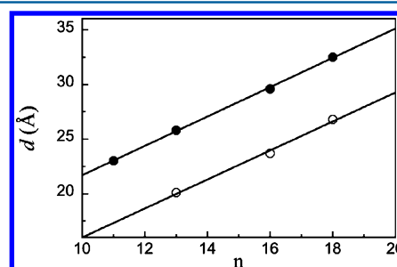
Figure 3. Interlamellar distance d as a function of n , the length of the 4- n -alkyl substituent on the triazole ligand, for the series \text{ZnC}_n\text{Cl} in the solid crystalline state (empty circles) and in the mesophase at 430–440 K (full circles).
