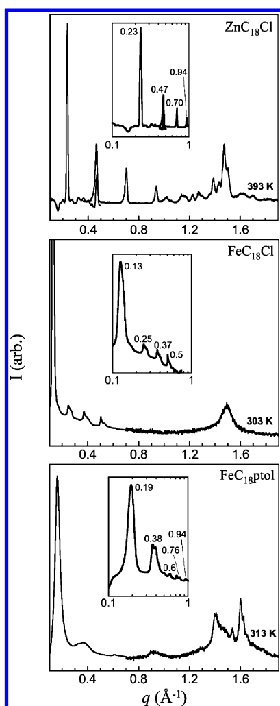
Figure 2. X-ray powder diffraction patterns in the (crystalline) solid state for \text{ZnC}_{18}\text{Cl} (top), \text{FeC}_{18}\text{Cl} (middle), and \text{FeC}_{18}\text{ptol} (bottom). Exact temperatures are indicated in each graph. Insets show the log–log plot of the low angle area. Data are taken from two separate measurements on two experimental set ups for small-angle and wide-angle ranges (see Experimental Section).
