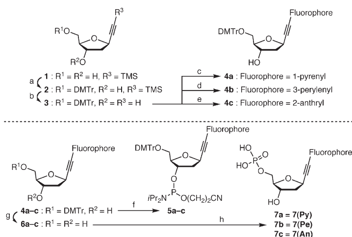
Scheme 2. a) 4,4'-Dimethoxytrityl chloride, 4-( N,N -dimethylamino)pyridine, pyridine; b) n Bu 4 NF, H 2 O, THF; c) 1-bromopyrene, [Pd(PPh 3 ) 4 ], CuI, i Pr 2 NH, THF; d) 3-bromoperylene, [Pd(PPh 3 ) 4 ], CuI, i Pr 2 NH, THF; e) 2-bromoanthracene, [Pd(PPh 3 ) 4 ], CuI, i Pr 2 NH, THF; f) NC-(CH 2 ) 2 OPCIN( i Pr) 2 , i Pr 2 NEt, CH 2 Cl 2 ; g) p -toluenesulfonic acid monohydrate, CH 2 Cl 2 ; h) phosphorus oxychloride, dioxane, pyridine.
