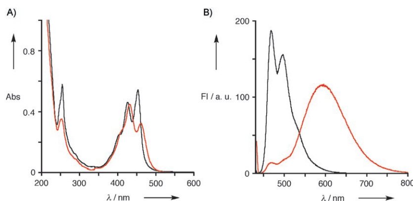
Figure 2. Absorption (A) and fluorescence (B) spectra of 7(Pe) (black line) and ab-Pe-Pe-ab (red line) in \text{H}_2\text{O} at 25^\circ\text{C} (FI = fluorescence intensity). Concentrations: [\text{7(Pe)}] = 2.0 \times 10^{-5} \text{ M} , [\text{ab-Pe-Pe-ab}] = 1.0 \times 10^{-5} \text{ M} . Excitation wavelength is 430 nm.
