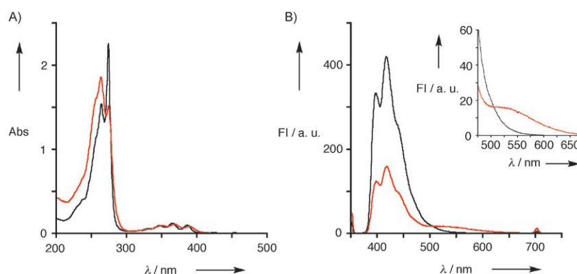
Figure 3. Absorption (A) and fluorescence (B) spectra of 7(An) (black line) and ab-An-An-ab (red line) in \text{H}_2\text{O} at 25^\circ\text{C} (FI = fluorescence intensity). Concentrations: [\text{7(An)}] = 2.0 \times 10^{-5} \text{ M} , [\text{ab-An-An-ab}] = 1.0 \times 10^{-5} \text{ M} . Excitation wavelength is 350 nm. The inset expands the region of the excimer emission.
