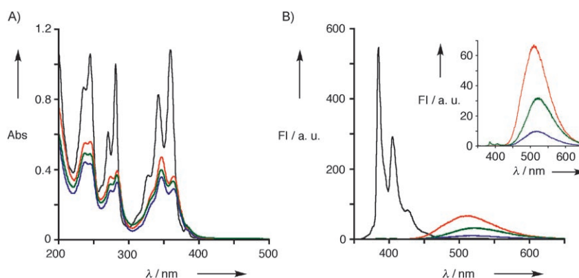
Figure 1. Absorption (A) and fluorescence (B) spectra of 7(Py) (black line), ab-Py-Py-ab (red line), ab-Py-Py-Py-ab (green line), and ab-Py-Py-Py-Py-ab (violet line) in H 2 O at 25°C (FI = fluorescence intensity). Concentrations: [\text{7(Py)}] = 2.0 \times 10^{-5} \text{ M} , [\text{ab-Py-Py-ab}] = 1.0 \times 10^{-5} \text{ M} , [\text{ab-Py-Py-Py-ab}] = 6.7 \times 10^{-6} \text{ M} , and [\text{ab-Py-Py-Py-Py-ab}] = 5.0 \times 10^{-6} \text{ M} . Excitation wavelength is 350 nm. The inset expands the region of the excimer emission.
