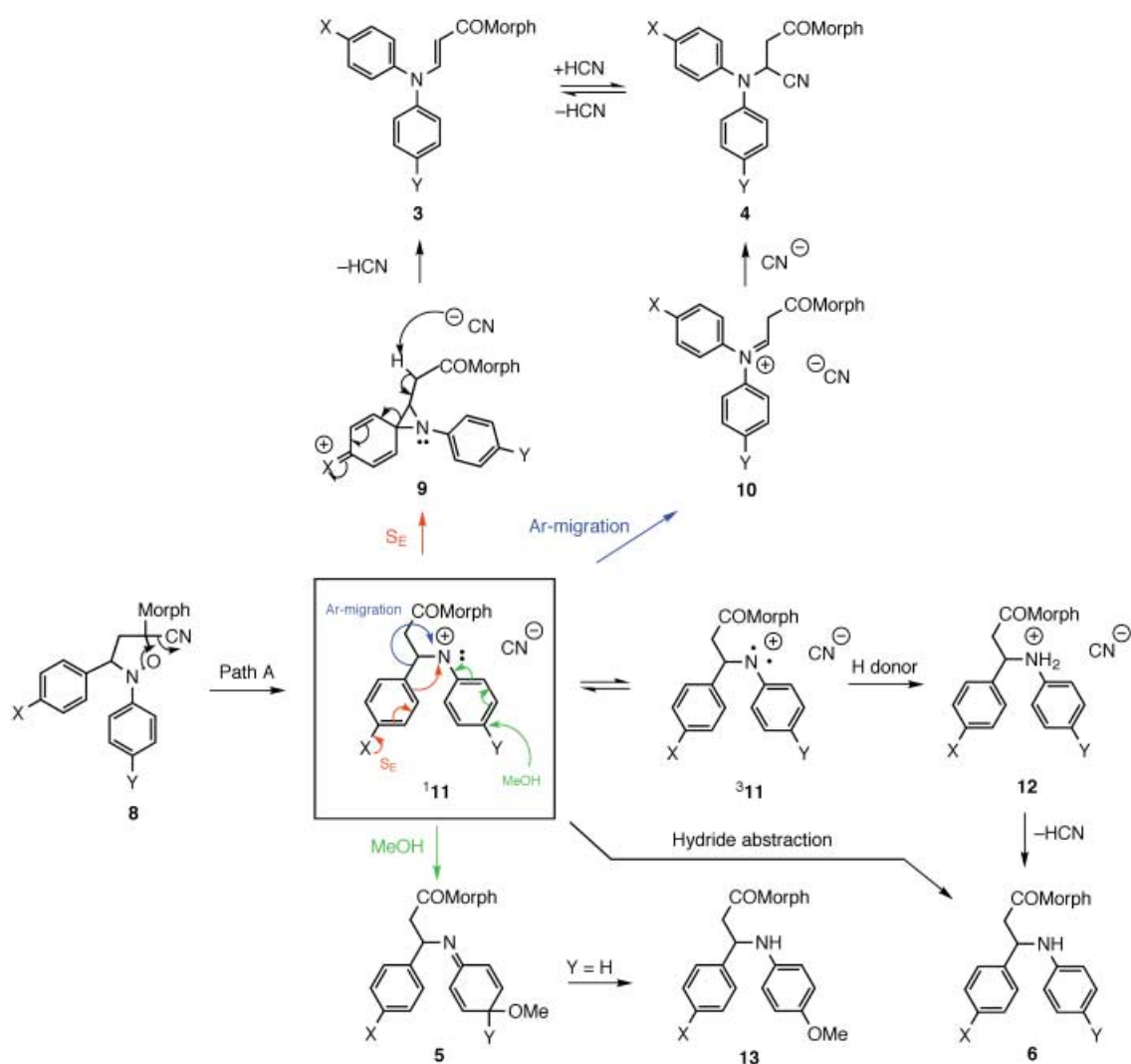
Scheme 4. Thermal rearrangement of isoxazolidines derived from C,N -diarylnitrones ( 1a-i ) and 2-morpholin-4-yl-acrylonitrile ( 2 ).
