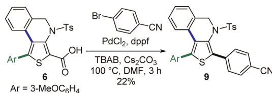
Scheme 3. Decarboxylative Cross-Coupling
