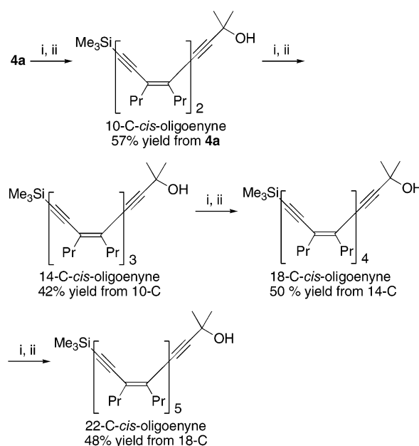
Scheme 4. Synthesis of cis -Oligoenynes a
