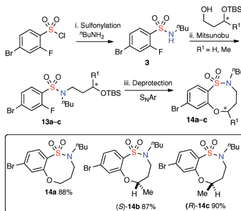
Scheme 3. Mitsunobu–Intramolecular S_NAr Strategy to Benzo-thiazocine-1,6-Dioxides a
