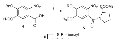
Scheme 1 Reagents and conditions: i , \text{SOCl}_2 L-proline methyl ester hydrochloride, \text{Et}_3\text{N} , \text{H}_2\text{O} , 0 °C, 30 min, 85%; ii , \text{BF}_3 \cdot \text{OEt}_2 –EtSH, \text{CH}_2\text{Cl}_2 , rt, 8 h, 88%.
