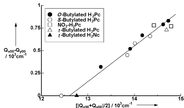
Figure 4. Correlation between the splitting of the Q band, Q_{x00} - Q_{y00} , and the mid-energy of the Q band (Q_{x00} + Q_{y00})/2 .
