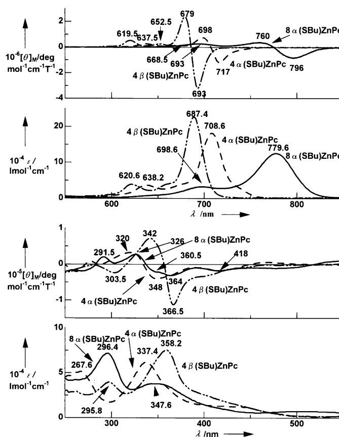
Figure 3. Electronic absorption and MCD spectra of 8α(SBu)ZnPc (solid lines), 4α(SBu)ZnPc (broken lines), and 4β(SBu)ZnPc (dotted broken lines) in THF in the Q (top) and B (Soret) band (bottom) regions.
