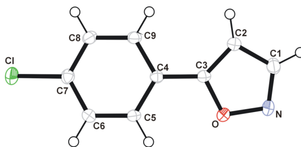
Figure 2. ORTEP of 5-(4-chlorophenyl)-isoxazole 4d ; reaction carried without the use of pyridine.
