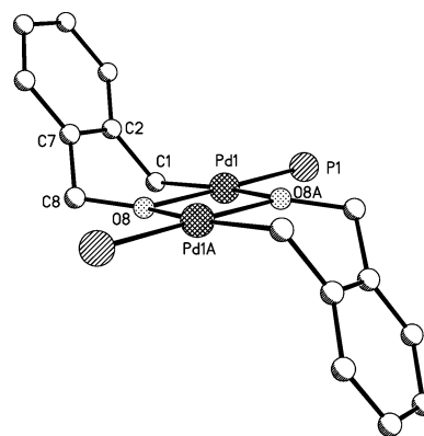
Figure 5. Structure around the five fused rings at the center of compound 7 .
