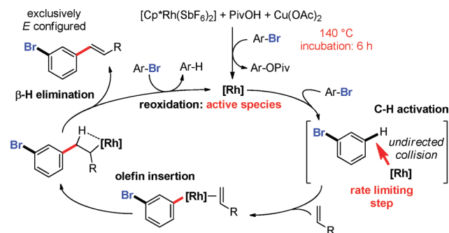
Scheme 2. Proposed Mechanism
