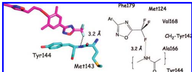
Figure 7. The 1,2,4-oxadiazole terminus of the rhinovirus blocker pleconaril sited in a hydrophobic pocket as determined by X-ray crystallography (1NCR). One of the CF 3 fluorine atoms engages in a slightly elongated hydrogen bond with the backbone NH of Tyr144.
