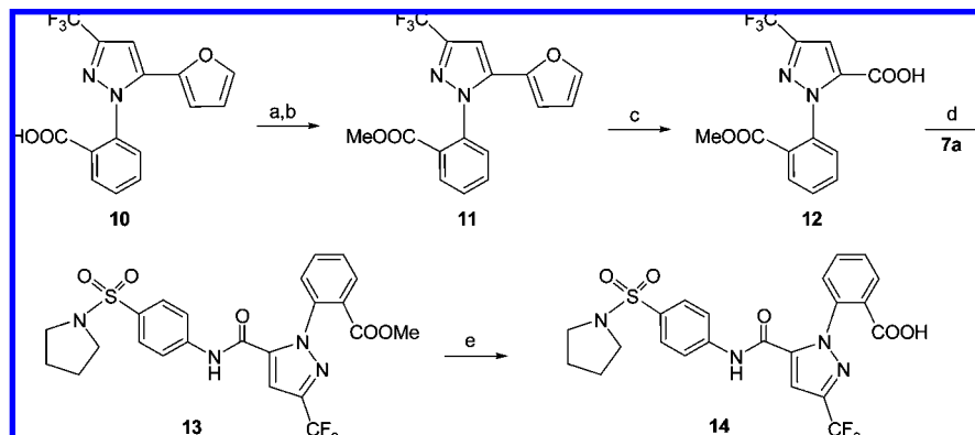
Scheme 3. Synthesis of 1-[2-Carboxy-phenyl]-3-trifluoromethyl-pyrazole Analogues a
