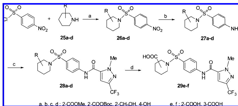
Scheme 5. Synthesis of Substituted Piperidine Derivatives 28 and 29 a
