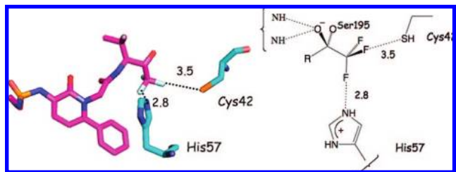
Figure 9. A trifluoromethyl ketone inhibitor of human leukocyte elastase (1EAS) illustrating an F—HS hydrogen bond and a charge dipole interaction between a ligand C—F bond and His57. Units for numerical values are Å.
