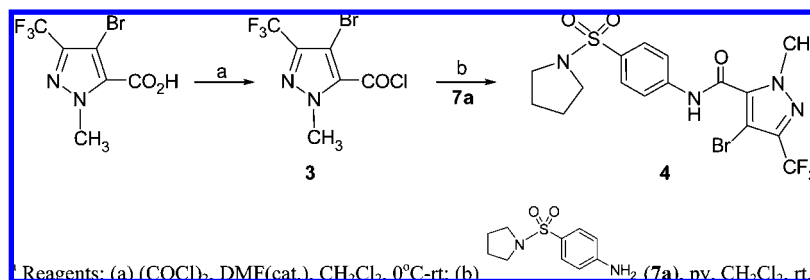
Scheme 2. Synthesis of 1-Alkyl-3-(trifluoromethyl)-5-carboxamide 9 a
