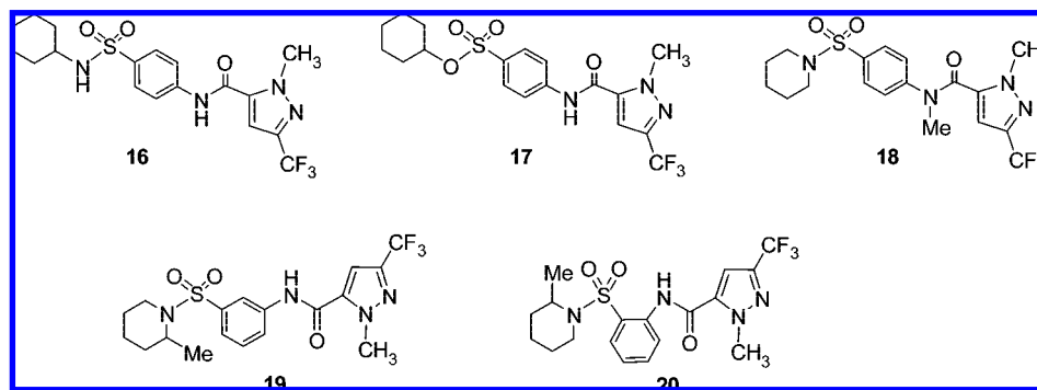
Figure 3. Variation scaffolds of piperidine analogues.
