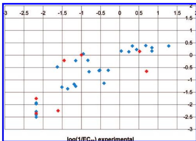
Figure 5. MFTA correlation for the 26 compounds of the training set (blue) and the seven compounds of the test set (red) based on charge ( Q ), effective vdW radius ( R_e ), and lipophilicity ( L_g ) descriptors.
