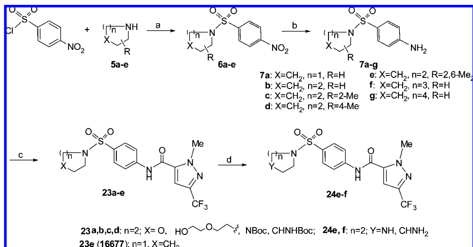
Scheme 4. Synthesis of Derivatives 23 and 24 a
