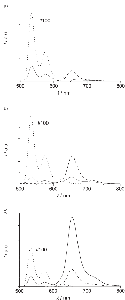
Figure 3. Room-temperature luminescence spectra in toluene of models and dyads excited at 490 nm. The luminescence of PI0 is divided by 100. a) C2 (---), PI0 (.....), C2-PI A = 0.12 (—); b) C3 (---), PI0 (.....), C3-PI A = 0.12 (—); c) C3 (---), PI0 (.....), C3-PPI A = 0.12 (—). The absorbance of the solutions are arranged to provide the same numbers of photons absorbed by the reference model and the same unit in the arrays.
