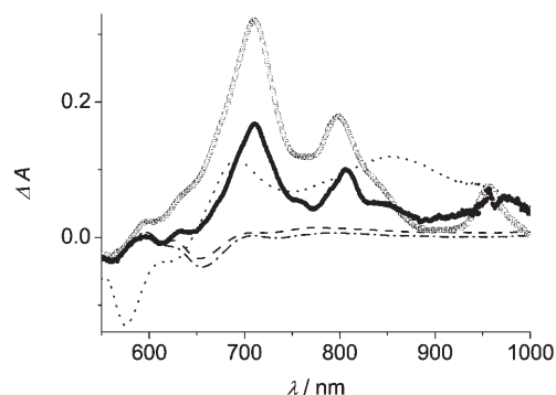
Figure 6. End-of-pulse absorption spectra of C2 (---) A=0.05 , C3 (---) A=0.05 , PI0 (....) A=0.43 , C3-PI A=0.6 (○), C3-PPI A=0.6 (●), C2-PI A=0.6 is superimposable on that of C3-PI and not shown. The absorbance of the solutions has been adjusted to provide the same light absorbance by the unit in the model and in the dyad.
