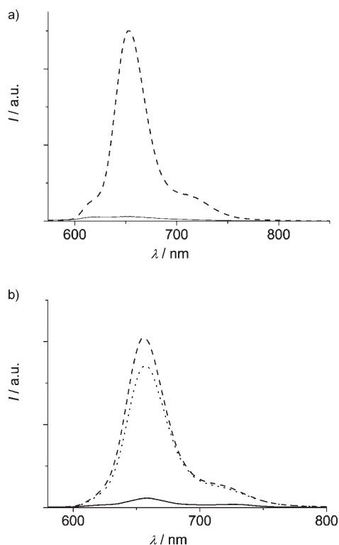
Figure 2. Room-temperature luminescence spectra in toluene of model corroles and dyads excited at 565 nm. a) C2 (---) and C2-PI (—) A = 0.136 ; b) C3 (---), C3-PI (—), C3-PPI (.....) A = 0.133 .
