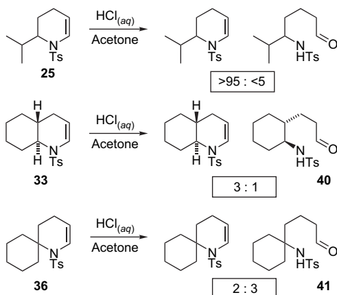
Scheme 4. Tetrahydropyridine stability.
