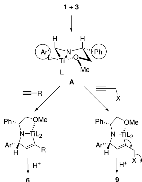
Scheme 4
