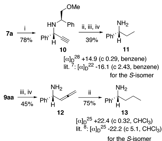
Scheme 3 a
