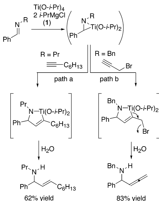
Scheme 1
