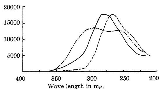
Fig. 2.—Spectra of the ionylideneacetic acids: —, \beta (solid); —, \beta (liquid); - - -, \alpha .
