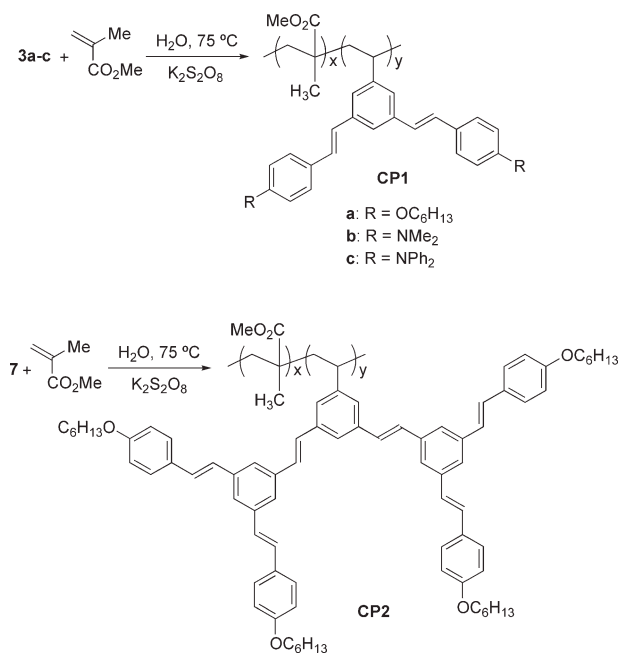
SCHEME 4 Copolymerization of PPV dendrons and MMA.
