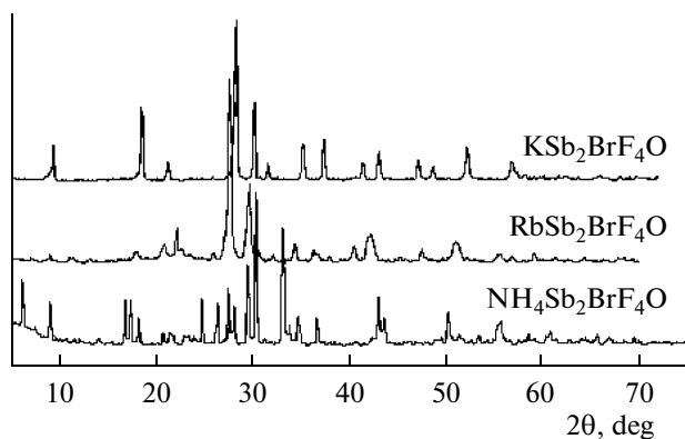
Fig. 1. Powder X-ray diffraction patterns for compounds synthesized.
