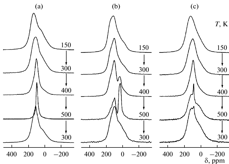
Fig. 5. Evolution of ^{19}\text{F} NMR spectra of (a) \text{KSb}_2\text{BrF}_4\text{O} , (b) \text{RbSb}_2\text{BrF}_4\text{O} , and (c) \text{NH}_4\text{Sb}_2\text{BrF}_4\text{O} in response to changing temperature.
