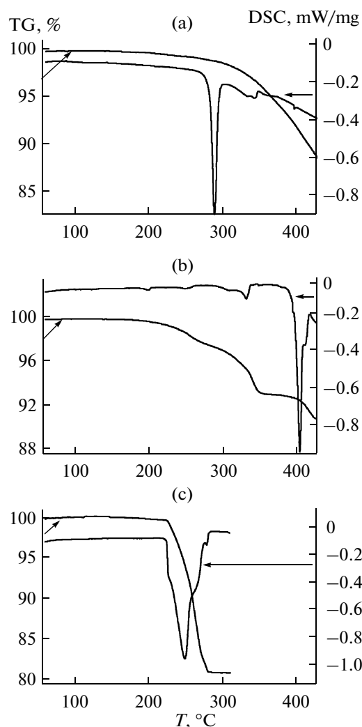
Fig. 4. Thermal curves for compounds synthesized: (a) \text{KSb}_2\text{BrF}_4\text{O} , (b) \text{RbSb}_2\text{BrF}_4\text{O} , and (c) \text{NH}_4\text{Sb}_2\text{BrF}_4\text{O} .
