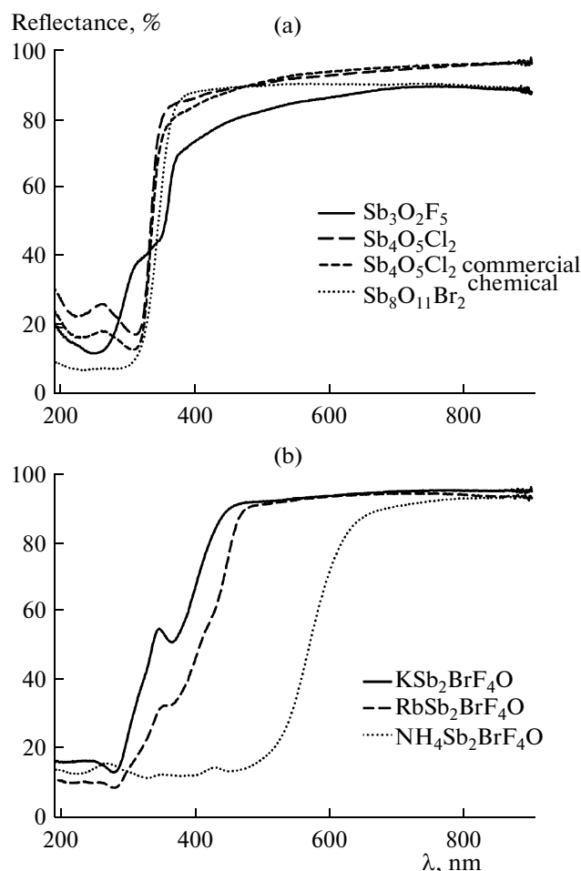
Fig. 3. (a) Optical reflectance spectra of (a) simple and (b) complex antimony(III) oxohalides.
