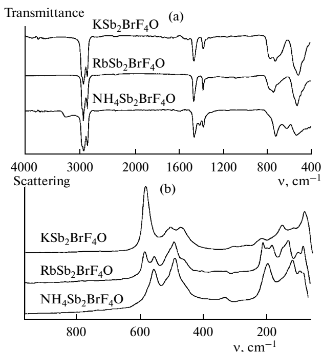
Fig. 2. (a) IR and (b) Raman spectra of compounds synthesized.
